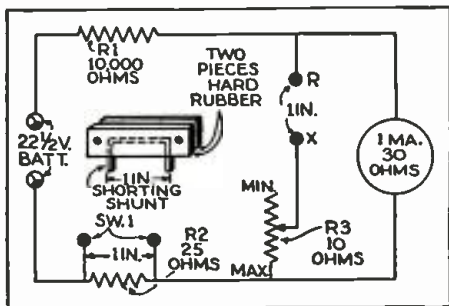
The circuit of the short ohmmeter.
