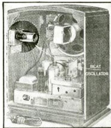
Fig. B. The unit installed in a G.E. set.
