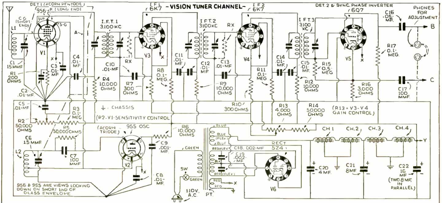
Fig. 1. The schematic of the video channel—the positions marked A, B, and C will be picked up in succeeding parts of the description.
