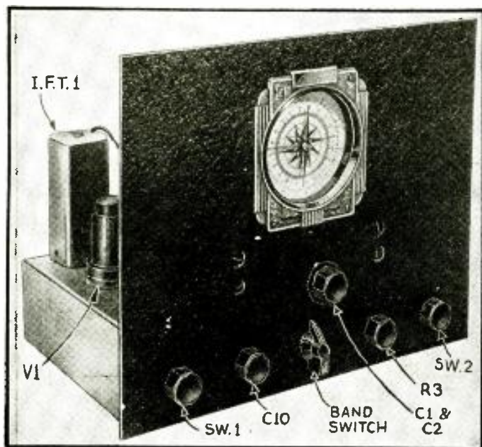
Fig. A. The panel of the converter with controls indicated.
